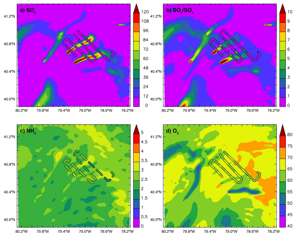
Fig. 5. Observed (tracks) and Domain 3 simulated (shading) values for (a) SO 2 , (b) SO 2 to aerosol sulfate ratio (c) aerosol ammonium ion, and (d) ozone. Aircraft observations are from the G-1 aircraft transect occurring 17:46 UTC to 18:30 UTC on 9 August at an altitude of 908 m above ground level (AGL). Simulated values are instantaneous model output at 18:00 UTC 9 August interpolated to the aircraft altitude. Units are parts-per-billion (ppb) for gaseous species and \mu\text{g m}^{-3} for aerosol species.
