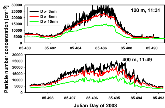
Fig. 10. Particle concentrations and horizontal variability for two selected flight levels on 26th March 2003.
