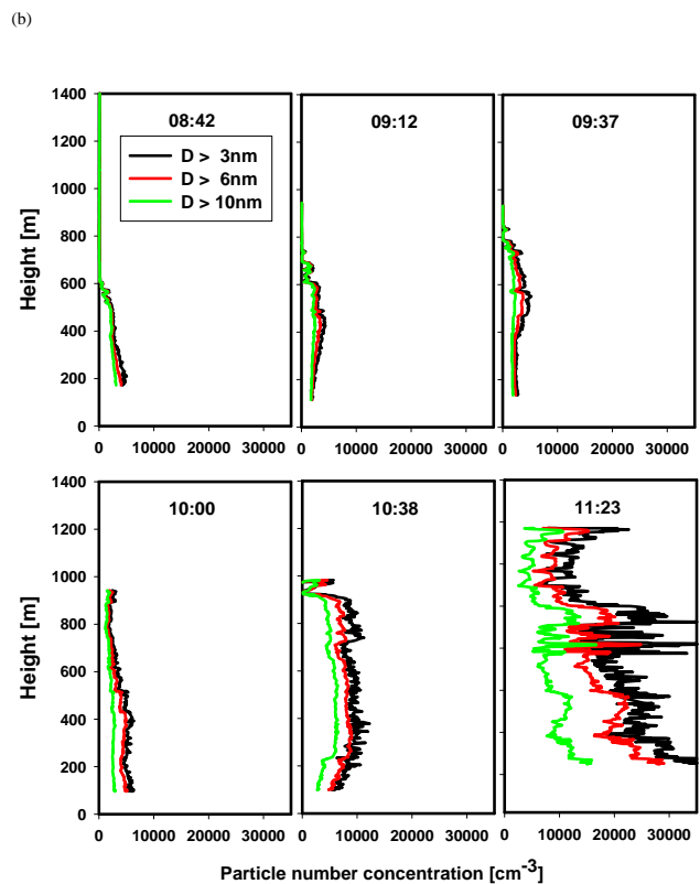
Fig. 12. (a) evolution of boundary layer structure, as determined by potential temperature and relative humidity, for 28th March 2003. (b) variation in aerosol vertical structure throughout the morning of 28th March 2003. Local time is also listed in each plot.
