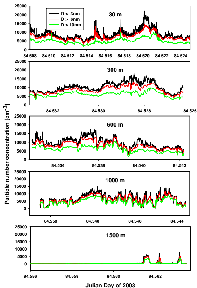
Fig. 7. Particle concentrations for 10 min horizontal runs at selected altitudes on 25th March 2003.
