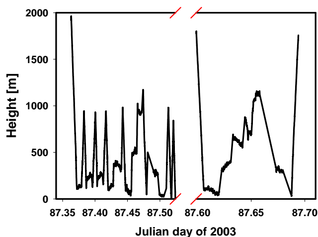
Fig. 11. Flight levels for 28th March 2003.
