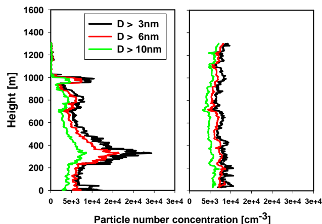
Fig. 6. Aerosol boundary layer structure for 25th March 2003. Total number concentration for sizes D > 3 nm, 6 nm and 10 nm. (Left) Aerosol concentration during descent from 11:53 to 12:04 local time and (Right) ascent at 13:51 to 13:49 local time. The latter profile indicates a more mixed aerosol field at the three sizes and indication that the free troposphere inversion has risen to > 1400 m.
