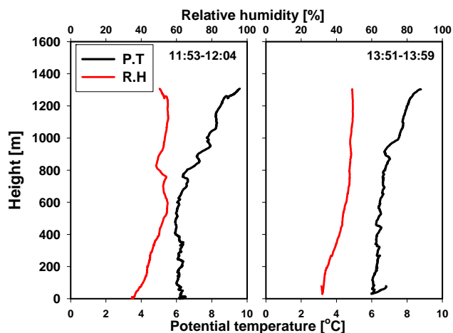
Fig. 5. Potential temperature (PT) and relative humidity (RH) boundary layer structure for 25th March 2003.
