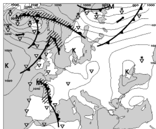
Fig. 3. Synoptic conditions on (a) 25th March 2003, (b) 26th March 2003 and (c) 28th March 2003.
