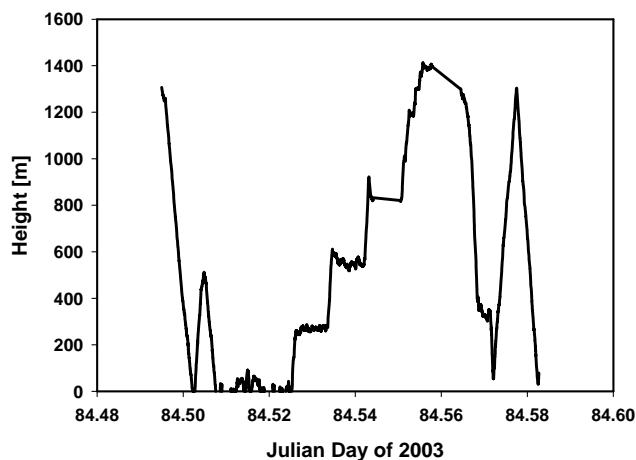
Fig. 4. Flight levels for 25th March 2003.
