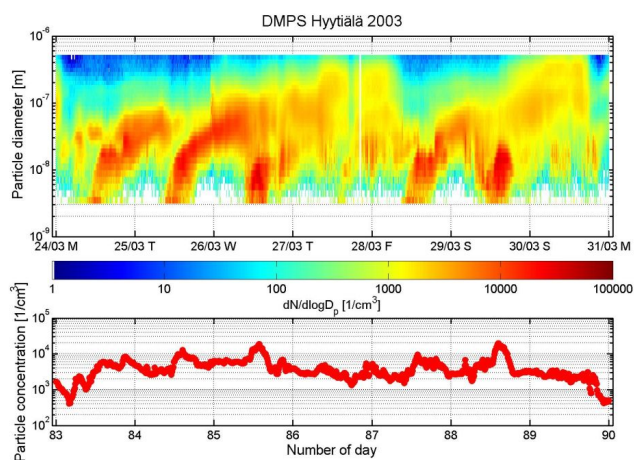
Fig. 2. Size distribution evolution during golden day nucleation events from 24th to 30th March 2003.
