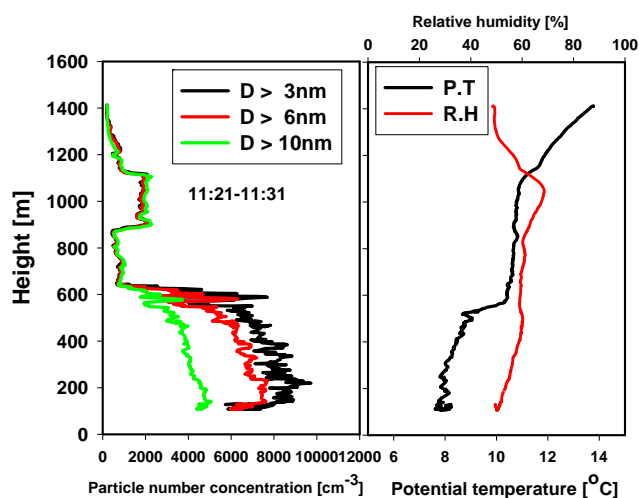
Fig. 9. Aerosol concentration potential temperature and relative humidity boundary layer structure on 26th March 2003.
