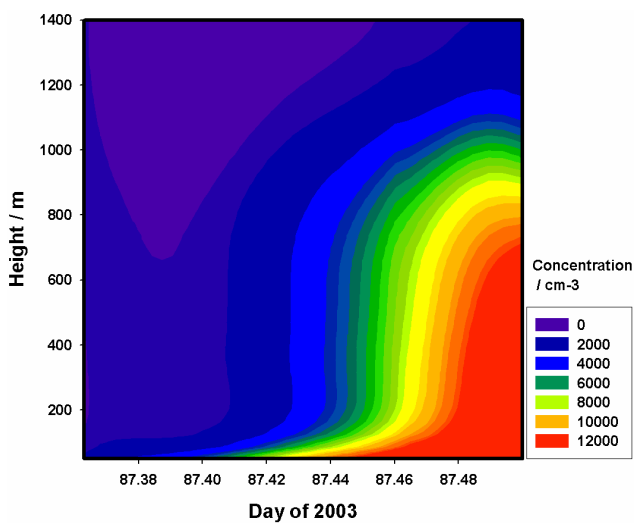
Fig. 14. Interpolated particle concentration at D > 3 nm for 24 profiles conducted on 28th March 2003.
