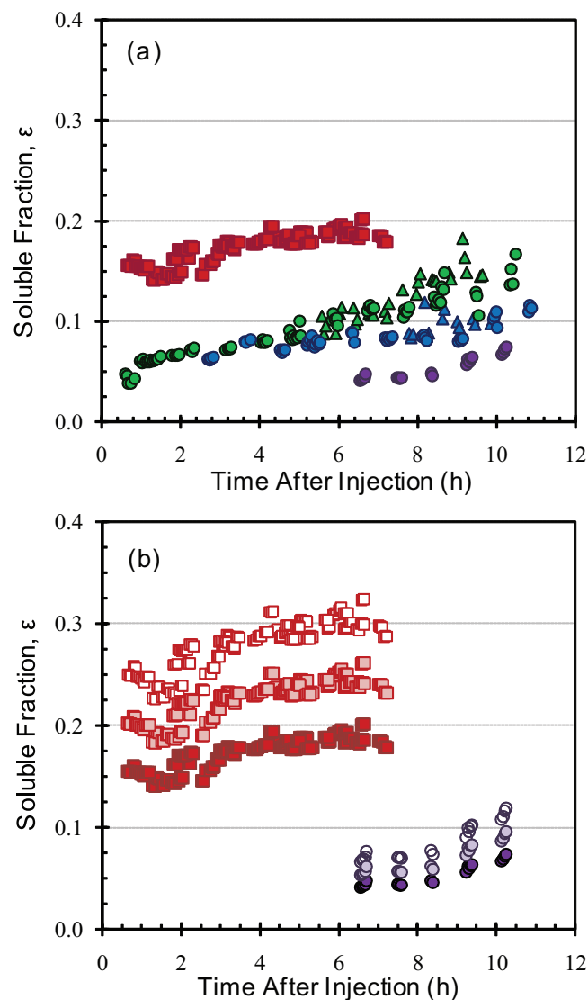
Fig. 7. Inferred soluble fraction as a function of aging for experiments 1, 2, 4 and 5. Square symbols represent SD measurements; circles and triangles represent CFTGC measurements for SOA formed in the presence and absence of OH, respectively. (a) \epsilon inferred assuming \sigma=66 m N m -1 and M_o=156 g mol -1 for SD measurements at 0.6% (red squares), CFTGC measurements at 1.02% (green symbols), 0.61% (blue symbols), and, for aerosol passed through the thermodenuder and exposed to 1.02% supersaturation (purple symbols). (b) Sensitivity of \epsilon to \sigma and M_o for data obtained with the SD (squares) and CFTGC (circles): \sigma=66 m N m -1 , M_o=156 g mol -1 (darkest closed symbols), \sigma=72 m N m -1 , M_o=156 g mol -1 (lightly shaded symbols), and, \sigma=66 m N m -1 , M_o=250 g mol -1 (open symbols).
