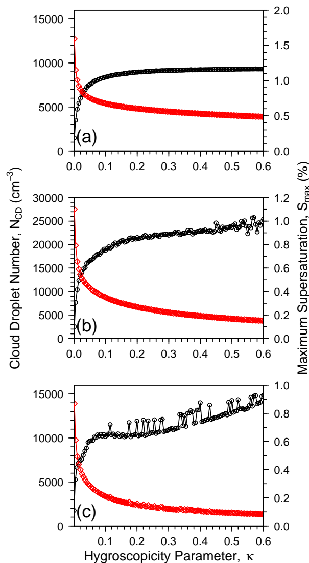
Fig. 8. Dependence of cloud droplet number concentrations ( N_{CD} , \text{cm}^{-3} , black) and maximum supersaturations ( S_{\max} , %, red) on aerosol particle hygroscopicity ( \kappa=0.005-0.6 ): (a) aerosol-limited regime ( w=15 \text{ m s}^{-1} and N_{CN}=1 \times 10^4 \text{ cm}^{-3} ); (b) aerosol- and updraft-sensitive (transitional) regime ( w=10 \text{ m s}^{-1} and N_{CN}=5 \times 10^4 \text{ cm}^{-3} ); (c) updraft-limited regime ( w=5 \text{ m s}^{-1} and N_{CN}=8 \times 10^4 \text{ cm}^{-3} ).
