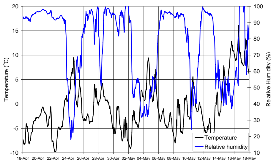
Fig. 5. Time series of temperature and relative humidity (RH) at Whistler Peak.
