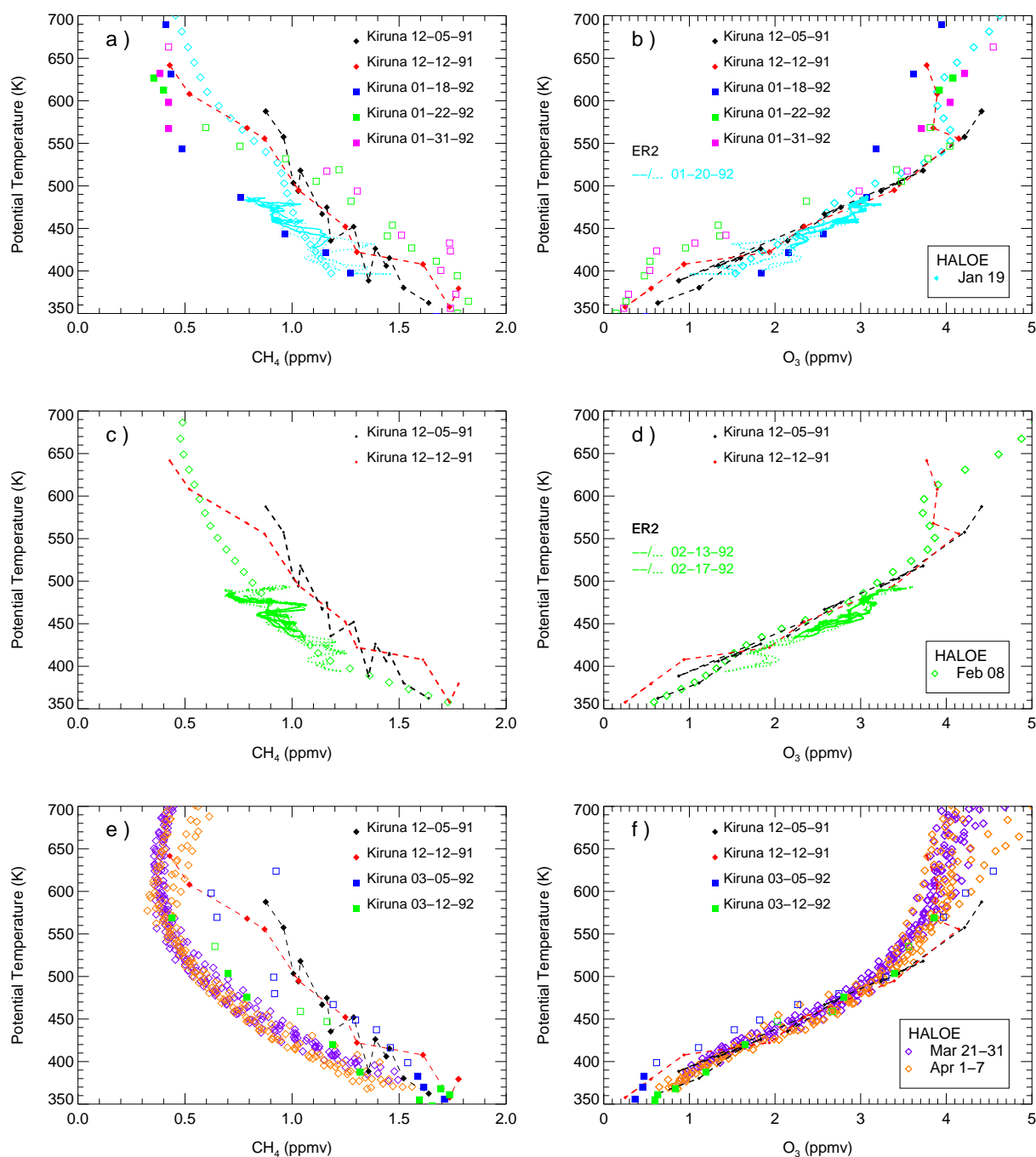
Fig. 3. \text{CH}_4 (left column) and \text{O}_3 (right column) mixing ratios with respect to potential temperature taken by the HALOE satellite, Kiruna balloons in the vortex core (filled symbols) and outside the vortex core (open symbols), and ER-2 aircraft observations within the vortex core (solid lines) and within the entire vortex (dotted lines), for different periods: January (top), February (middle) and March 1992 (bottom). Kiruna balloon observations during December (red and black symbols and dashed lines) are shown in each panel as early winter reference profiles.
