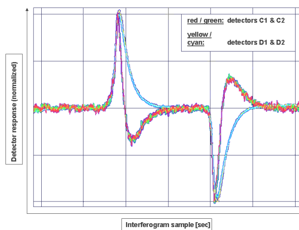
Fig. 8. In-orbit check of detector co-alignment (target: Mercury, date: 5 July 2002).
