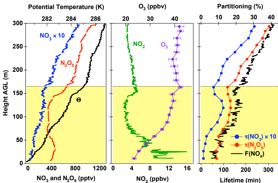
Fig. 7. Same as Fig. 6, except for a profile from 03:05–03:14. Note that \text{O}_3 is displayed against the top axis in the center graph in this figure. The layering color scheme is the same as for Fig. 5, except that the surface layer is absent.
