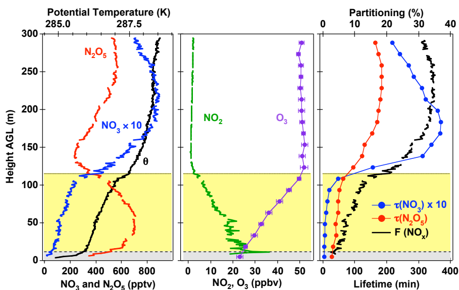
Fig. 6. Left: Profile of \text{NO}_3 and \text{N}_2\text{O}_5 (bottom axis), and potential temperature (top axis) as a function of height above ground level (AGL) from 23:15–23:23 on 4 October 2004. Note that the \text{NO}_3 mixing ratio has been multiplied by a factor of 10 to display it on the same scale with \text{N}_2\text{O}_5 . Center: Vertical profiles of \text{O}_3 (measured at 18 s time resolution) and \text{NO}_2 , calculated from the measured \text{NO}_3 , \text{N}_2\text{O}_5 and temperature according to Eq. (1). Right: Profile of \text{NO}_3 and \text{N}_2\text{O}_5 lifetimes (bottom axis) calculated according to Eq. (4) (with \tau(\text{NO}_3) multiplied by 10) and partitioning, F(\text{NO}_x) (top axis) from Eq. (5). The horizontal lines and color coding indicate the layer assignments according to the scheme shown in Fig. 5.
