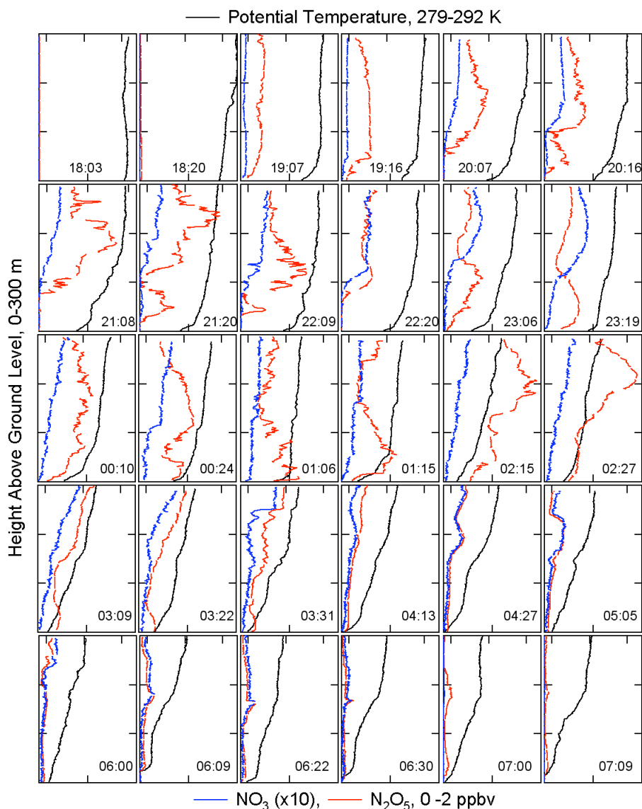
Fig. 4. Overview of 30 profiles from just prior to sunset to just after sunrise on 4–5 October. \text{NO}_3 (blue, multiplied by 10) and \text{N}_2\text{O}_5 (red) are shown against the bottom axis of each plot against a uniform scale from 0–2 ppbv. Potential temperature (black) is shown against the top axis of each plot on a uniform scale from 279–292 K. The left axes are altitude from 0–300 m. The time on each plot corresponds to the approximate midpoint of the profile.
