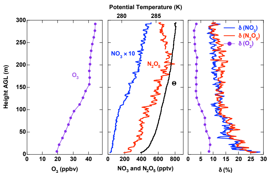
Fig. 9. Vertical profiles of averaged \text{O}_3 (left graph) \text{NO}_3 , \text{N}_2\text{O}_5 and potential temperature ( \Theta ) (center graph) for 27 profiles between 10 April 2004 19:00–10 May 2004 06:00. The relative standard deviation of \text{NO}_3 , \text{N}_2\text{O}_5 and \text{O}_3 (see text) are shown in the right graph. The apparently systematic oscillations in the averages are an artifact of the frequency at which zero measurements were taken during vertical ascents and descents.
