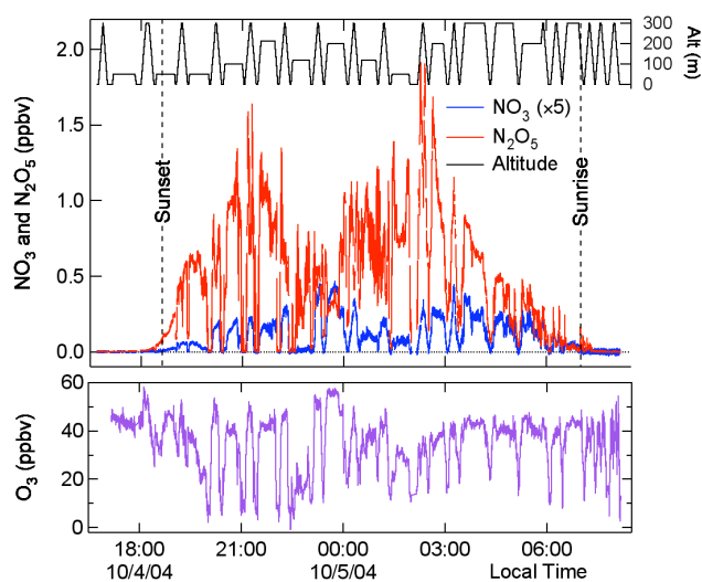
Fig. 2. Time series of the measured mixing ratios of NO 3 ( \times 5 ), N 2 O 5 (top graph) and ozone (bottom graph). The altitude derived from the pressure measurements appears above the top graph against the right axis. Approximate times of local sunrise and sunset (i.e., solar zenith angle = 90° at the surface) are marked.
