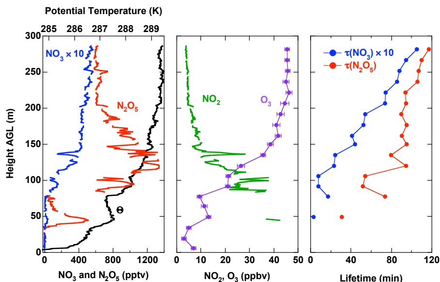
Fig. 8. Same as Fig. 6, except for a profile from 22:05–22:14.
