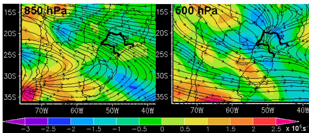
Fig. 1. 8 February 2001 at 00:00 UT: Streamflow lines and divergence (in s^{-1} ) at 850 hPa (left panel) and 500 hPa (right panel), with borders of the State of São Paulo shown in bold, from CPTEC Global analysis.
