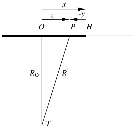
Fig. 1. Geometry of trail and radar scattering.
