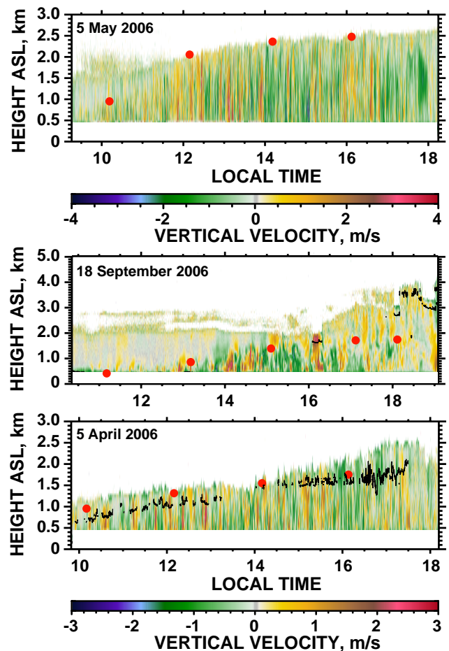
Fig. 1. Evolution of the ABL in terms of vertical velocity observed with Doppler lidar (resolution: 5 s, 75 m) at Leipzig on 5 May 2006 (top), 18 September 2006 (center), and 5 April 2006 (bottom). Yellow and red (positive velocities) indicate upward movements, whereas green and blue (negative velocities) represent downward movements. Red circles show the general trend in the increase of the ABL top height as observed with an automated aerosol lidar. Cloud base heights of convective clouds are indicated by black lines. Lidar signals from the near range (region of detector saturation) are not trustworthy and thus not shown. 12:00 Local Time (LT, daylight saving time) is 11:00 Central European Time (CET) and 10:00 UTC.
