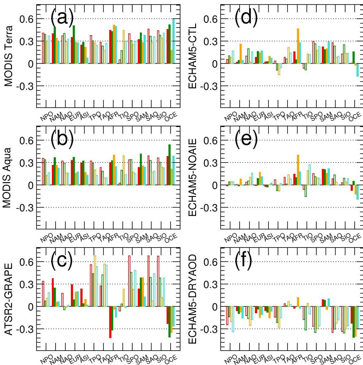
Supplementary Fig. 2. Slopes of the relationship \ln TCC vs. \ln AOD, for (a) MODIS Terra, (b) MODIS Aqua, (c) ATSR2-GRAPE, (d) ECHAM5 control simulation, (e) ECHAM5 simulation without aerosol indirect effects, and (f) as (e), but using dry rather than humidified AOD. The slopes for the individual regions are shown (abbreviations as in Supplementary Fig. 1), with oceanic regions in open, land regions in filled bars. Colours show the different seasons: Red – December-January-February, Green – March-April-May, Yellow – June-July-August, Turquoise – September-October-November.
