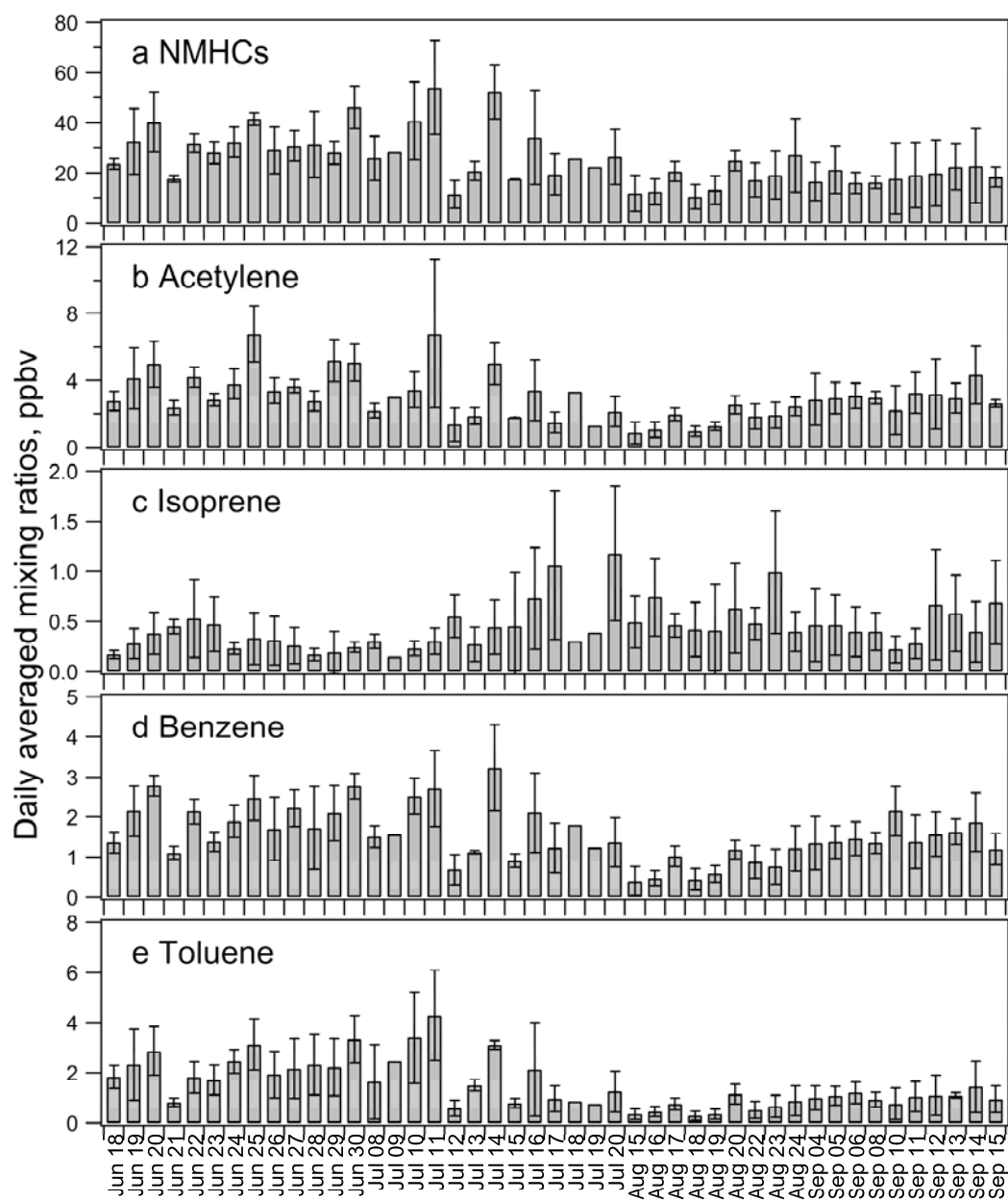
Figure S1. Daily averaged mixing ratios of (a) NMHCs, (b) acetylene, (c) isoprene, (d) benzene, and (e) toluene at PKU site. The error bars are standard deviations.
