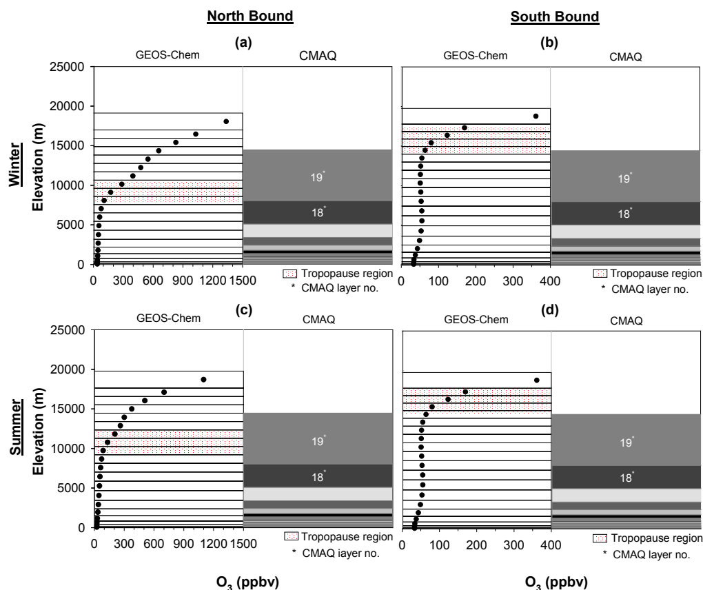
Fig. 5. Vertical ozone profiles from GEOS-Chem plotted with GEOS-Chem and CMAQ layers for both summer and winter, (a) north bound in winter, (b) south bound in winter, (c) north bound in summer, and (d) south bound in summer.
