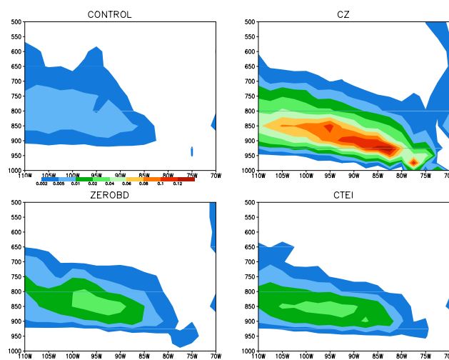
Fig. 5. Vertical cross-section of monthly mean cloud water in July along 20S.
