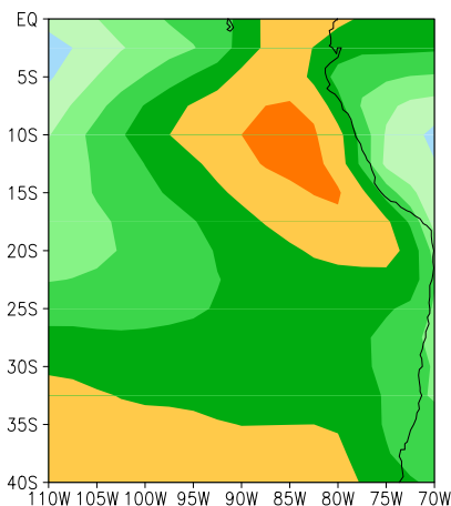
Fig. 2. The ISCCP July mean (1985–1993) total cloudiness in July in the SEP region.
